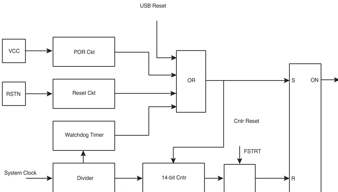
Figure 6. Reset Logic
